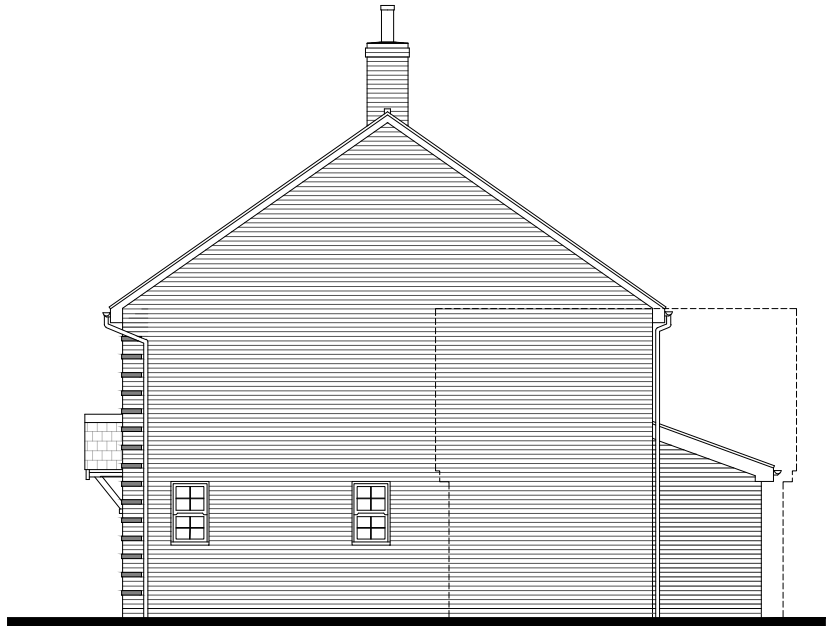
PLOT 2 SIDE ELEVATION
