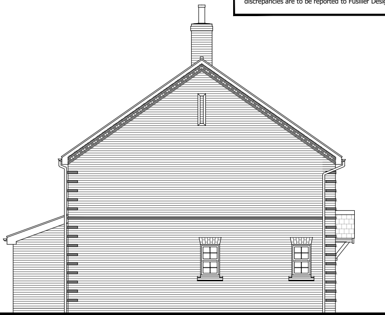
PLOT 1 SIDE ELEVATION
